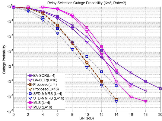
Fig. 3 Outage probability for K=8, L=4, 16, \gamma_0=2 .
