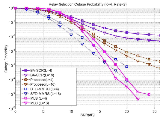
Fig. 2 Outage probability for K=4, L=4, 16, \gamma_0=2 .
